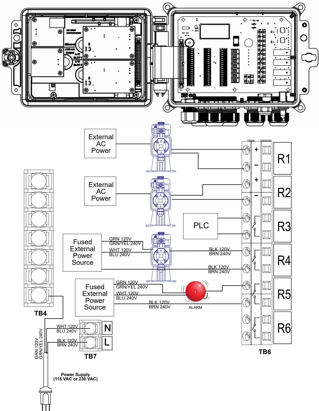
Figure 16 W620 AC Power & Relay Output Wiring
